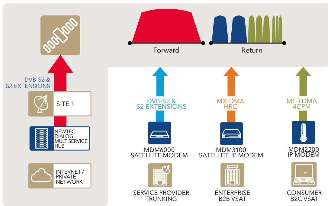
Figure 12: Newtec Dialog multiservice platform with shared hub for SCPC, MF-TDMA and Mx-DMA terminals
