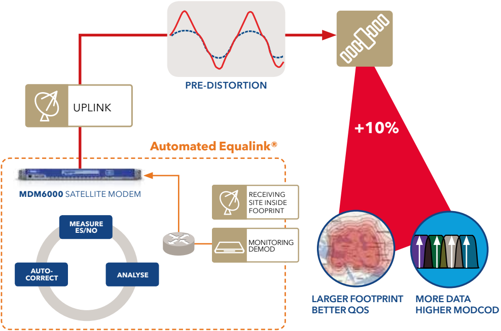
Figure 9: Efficiency technologies Bandwidth Cancellation and Automated Equalink to further optimize the satellite link
