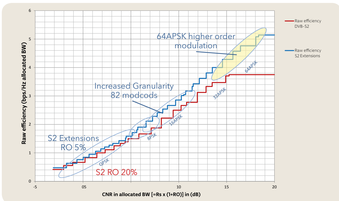
S2 Extensions with RO 5% compared to DVB-S2 with RO 20%
