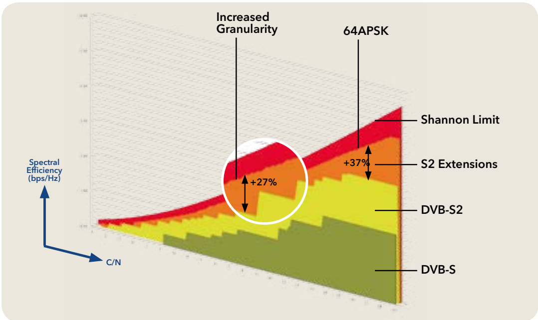
S2 Extensions compared to DVB-S2 (64APSK & increased granularity)
